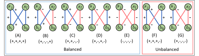
Figure 2: Undirected Signed Butterfly Isomorphism Classes.
